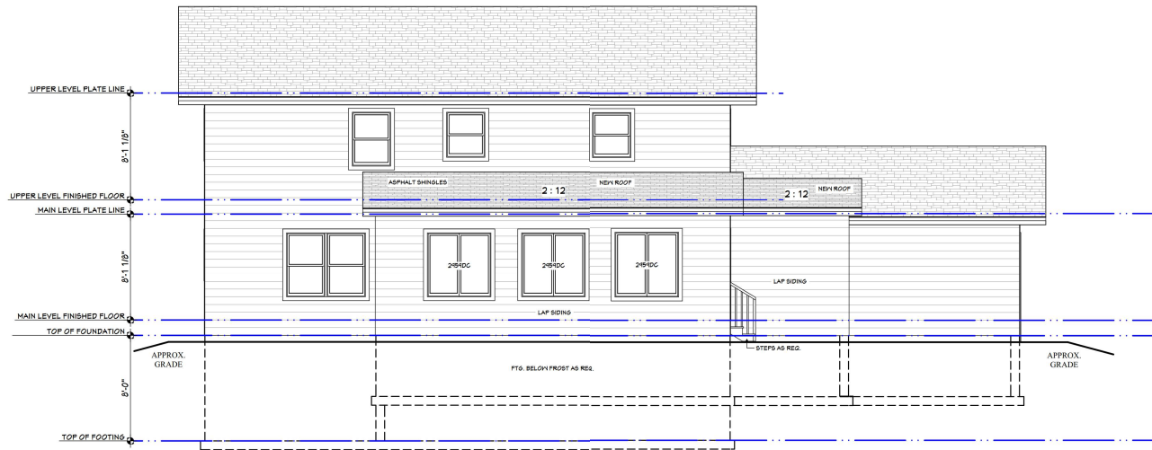
NEW REAR ELEVATION SCALE: 1/4" = 1'-0"
