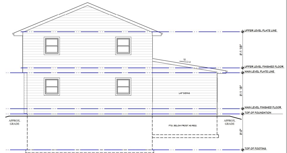
NEW RIGHT ELEVATION SCALE: 1/4" = 1'-0"
