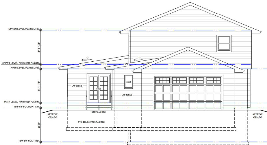
NEW LEFT ELEVATION SCALE: 1/4" = 1'-0"
