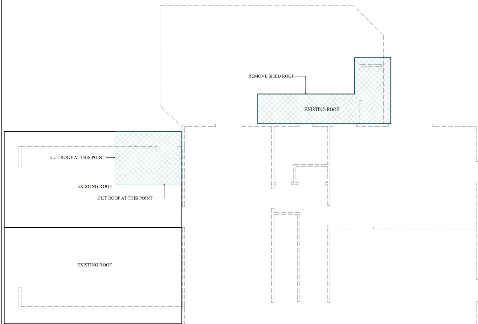
MAIN LEVEL EXISTING/DEMO ROOF PLAN SCALE: 1/4" = 1'-0"
