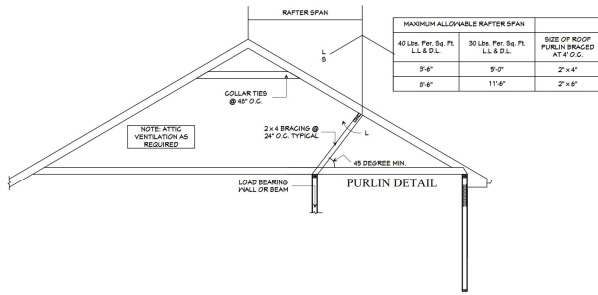
PURLIN DETAIL SCALE: 1/4" = 1'-0"
