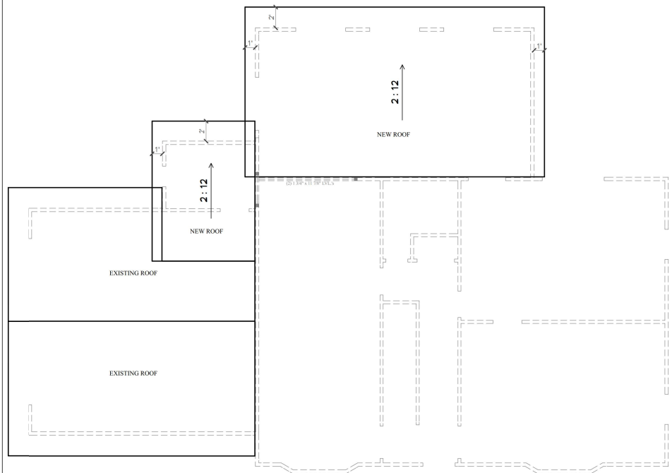
NEW MAIN LEVEL ROOF PLAN SCALE: 1/4" = 1'-0"
