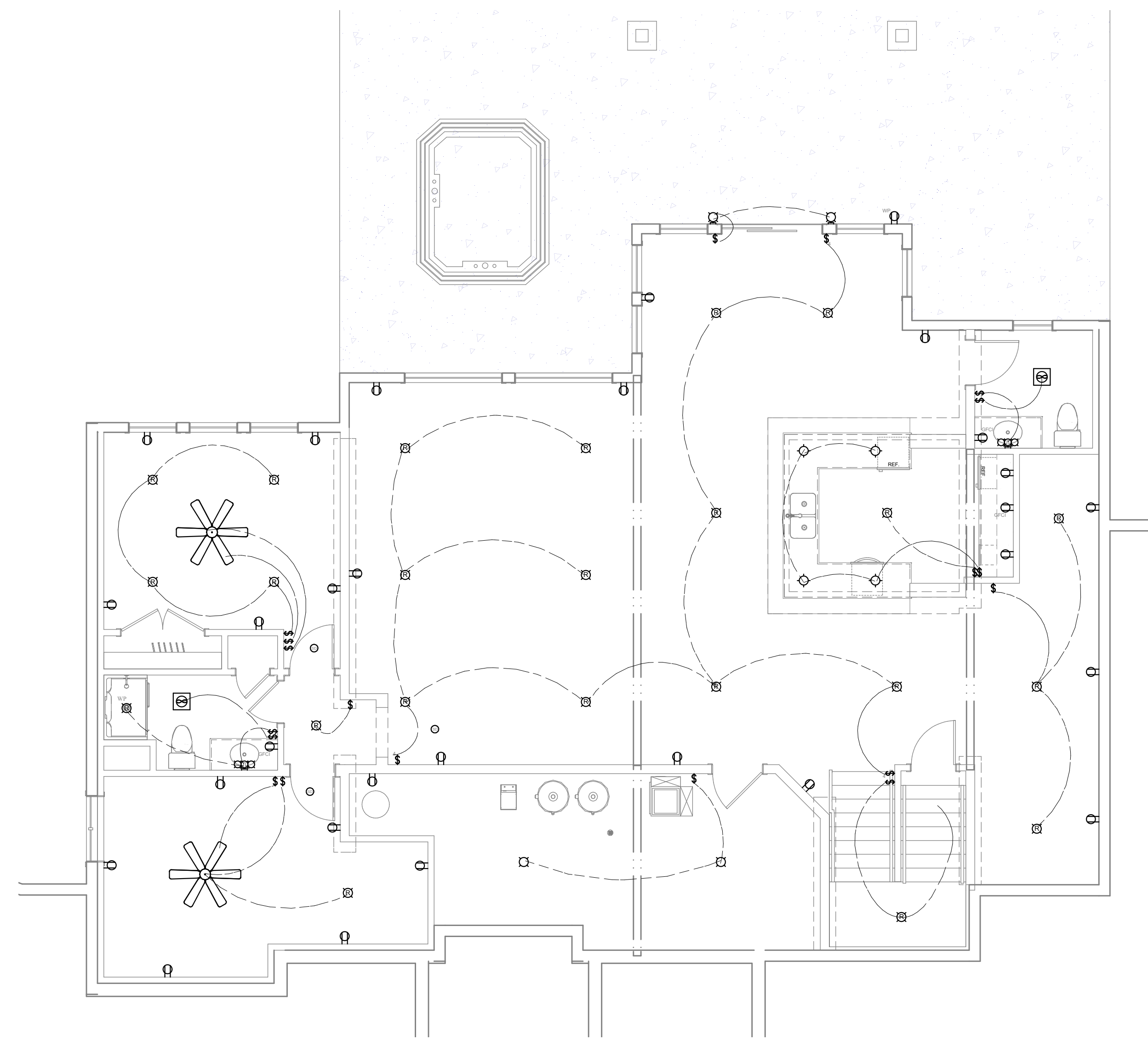
BASEMENT ELECTRICAL PLAN
