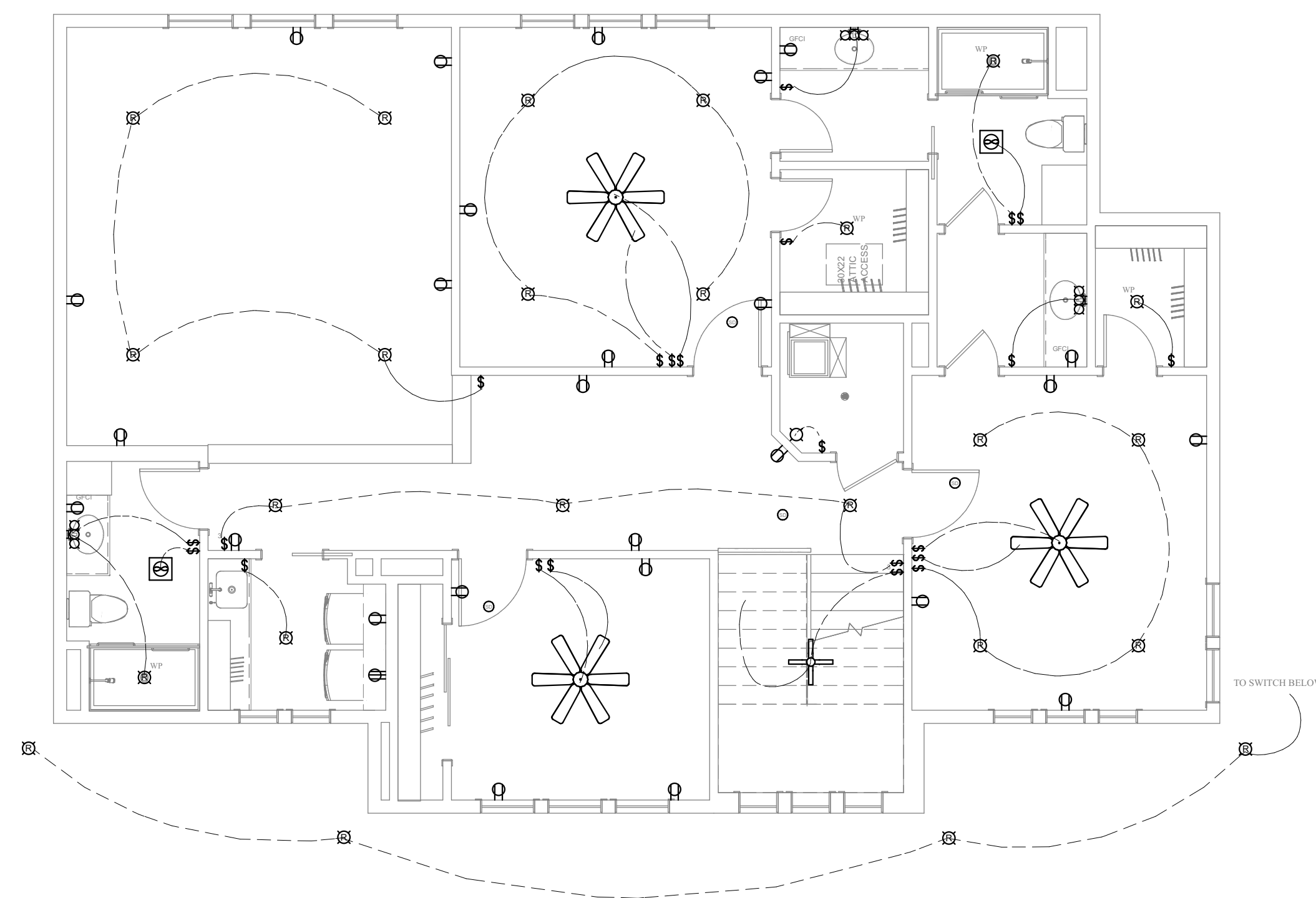
UPPER LEVEL ELECTRICAL PLAN
