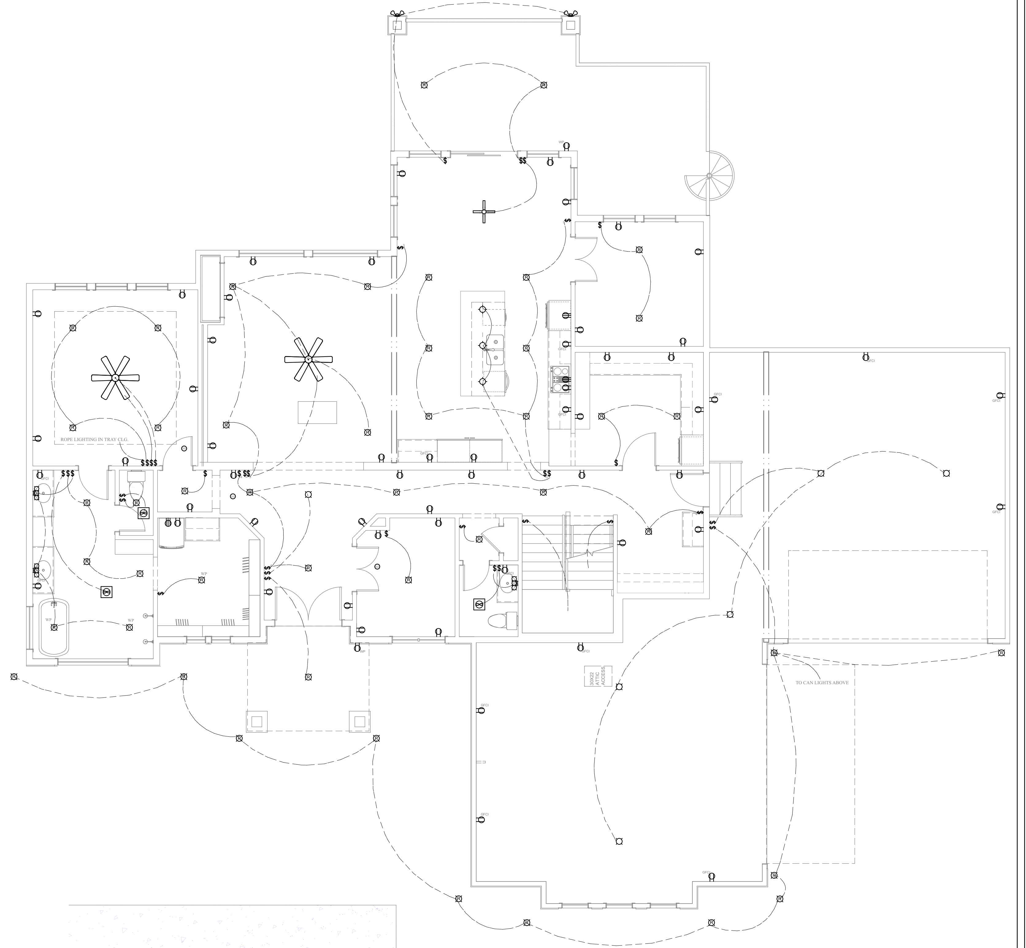
MAIN FLOOR ELECTRICAL PLAN
