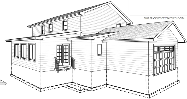
NEW REAR-RIGHT 3D PERSPECTIVE VIEW
