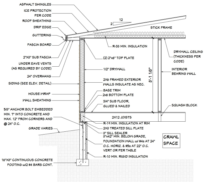
ADDITION WALL SECTION SCALE: 1/2" = 1'-0"
