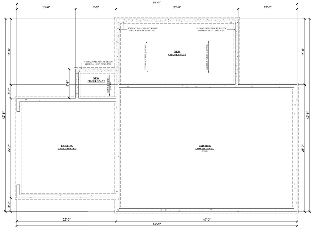
NEW BASEMENT/FOUNDATION PLAN SCALE: 1/4" = 1'-0"
